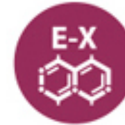
SULPHUR DIOXIDE
